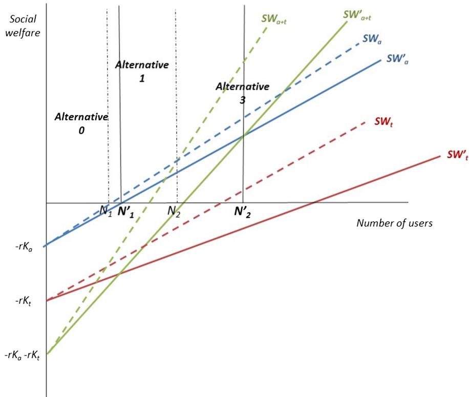
Fig. 4. Optimal alternative depending on the charging scheme.
