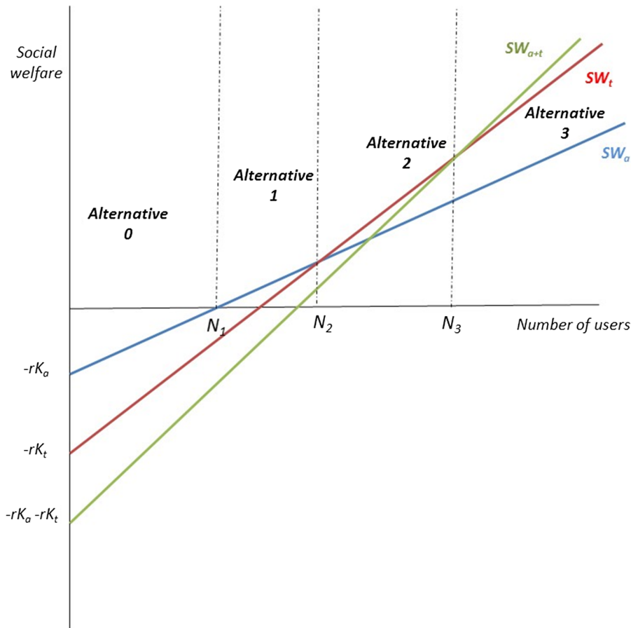
Fig. 1. Optimal alternative depending on the number of users in the economy: Example 1.
