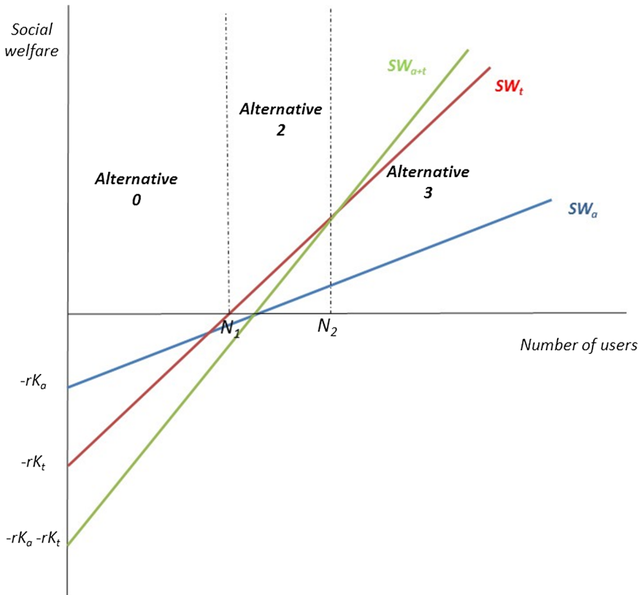
Fig. 3. Optimal alternative depending on the number of users in the economy: Example 3.
