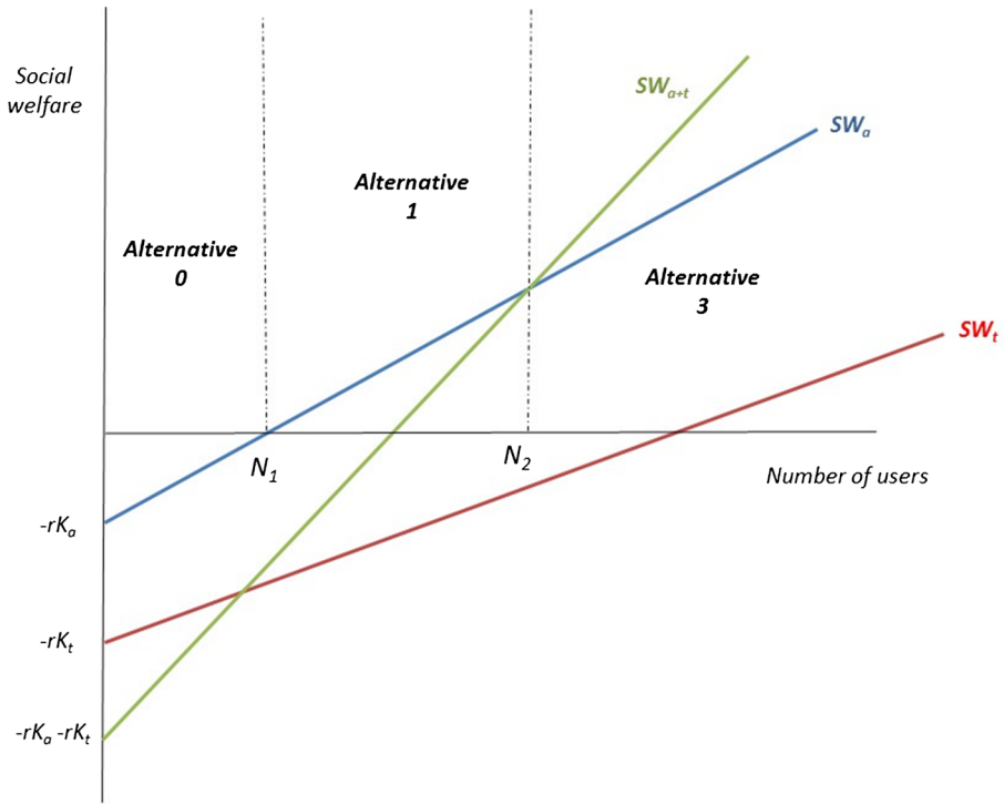
Fig. 2. Optimal alternative depending on the number of users in the economy: Example 2.
